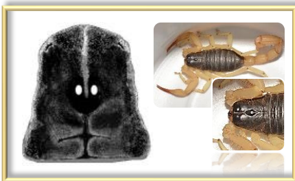
Hadrurus Spadix
